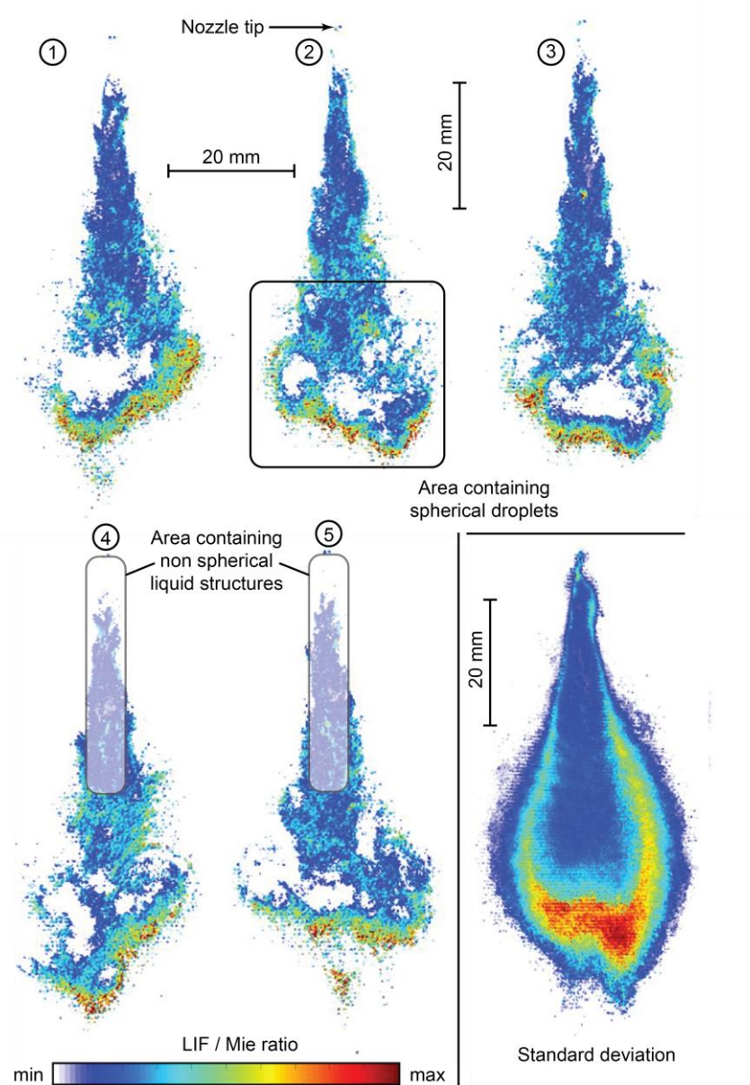
Fig. 10 Comparison of five single-shot images of the LIF/Mie ratio at 2300 \mu s after the electrical start of injection for an ethanol spray generated by a 5-holes DISI-injector (adapted from [26]).
