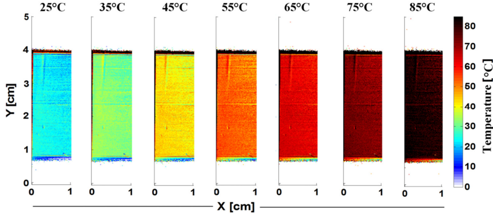
Fig. 8. Calibrated SLIPI-LIF ratio depicting the absolute temperature of the liquid in the cuvette. Results have been deduced using the SLIPI calibration curve given in Fig. 7. It is seen that the water temperature is nearly homogenous throughout the cuvette for each reference temperature case ranging between 25°C to 85°C.
